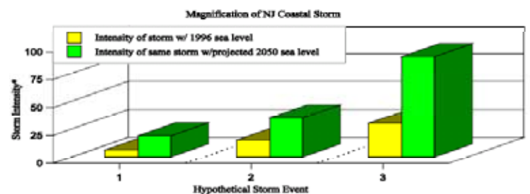
Figure 1. Increasing Intensity of Coastal Storms in New Jersey With Climate Change
